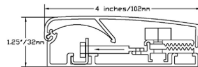
Banner Grip frame dimensions
